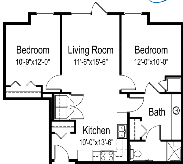
Floor plan B2 Two bedrooms, one bathroom 865 square feet
