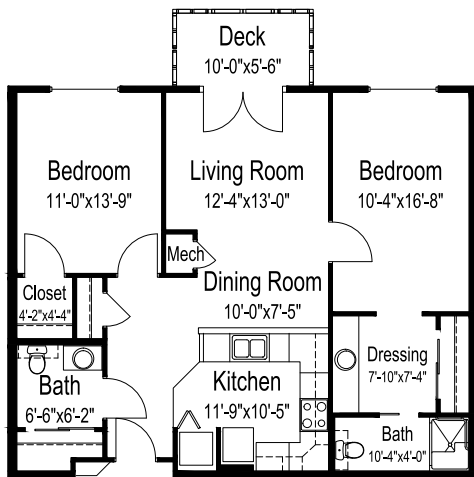
Two bedrooms, one and one-half bathrooms
